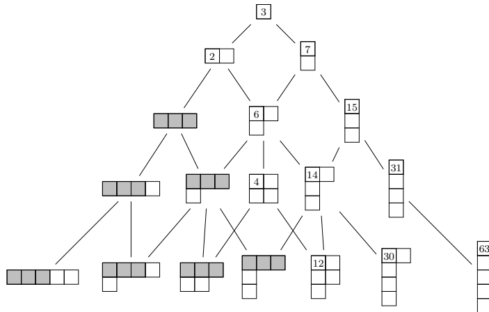
Figure 1: The Young lattice for the class of R-matrices associated to the pair (\emptyset, \begin{smallmatrix} \square & \square \\ \square & \square \end{smallmatrix}) . Since the length of the first partition is 0 and that of the second is 2, any diagram containing a rectangle of height 1 and width 3 gives multiplicity 0. The first irreducible representation whose corresponding partition contains such a rectangle is the trivial representation of S_3 . For the remaining diagrams the multiplicities are given in the first box.
